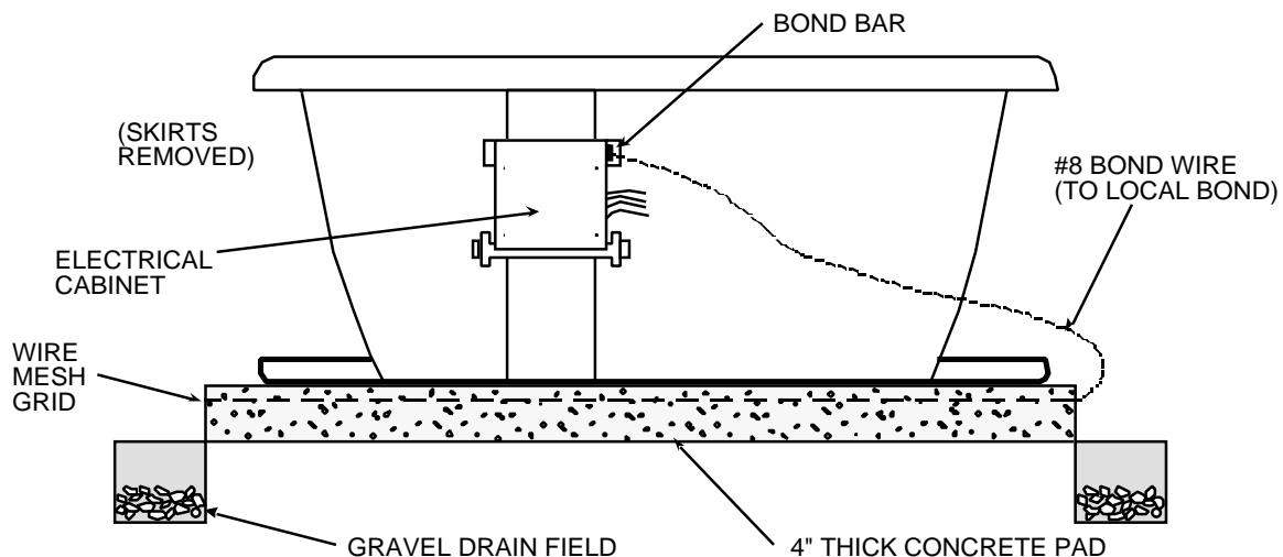
SUPPORT, DRAINAGE AND BONDING
